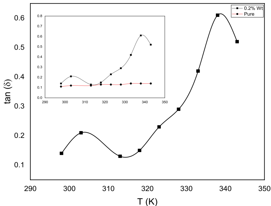
Fig. 4. Dielectric loss tangent ( \tan \delta ) versus temperature T(K) of PMMA doped with lithium chloride 0.2%wt.
