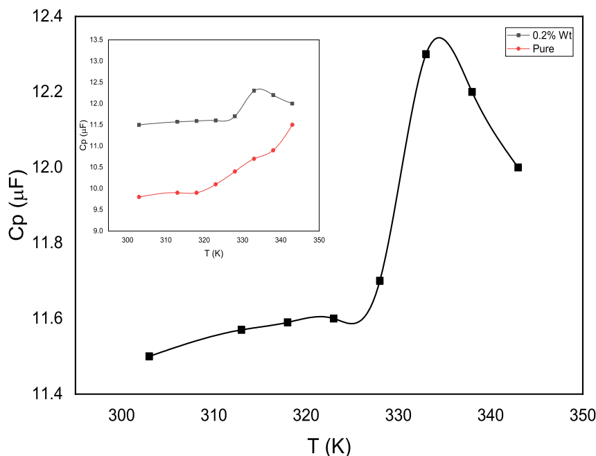
Fig. 1. Electrical capacity ( \mu\text{F} ) versus temperature T (K) of /LiCl.
