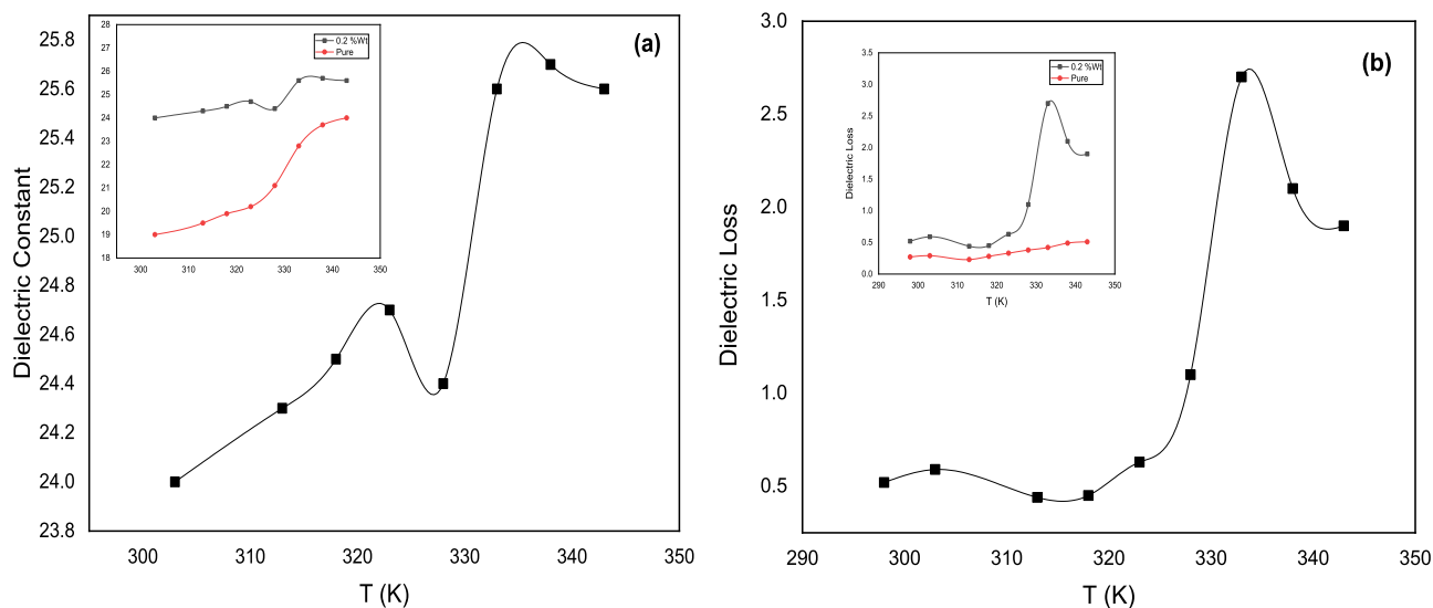
Fig. 3. (a) Dielectric constant \epsilon' and (b) Dielectric loss \epsilon'' as a functions of temperature T (K) for PMMA/LiCl.
