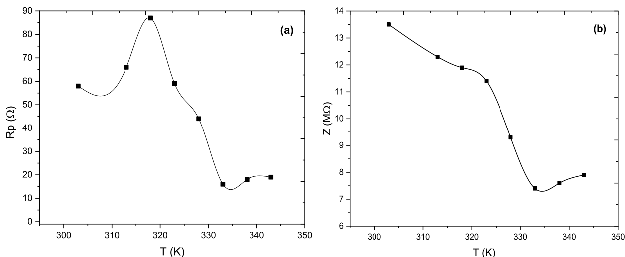
Fig. 2. (a) Resistance R_p ( \Omega ) and (b) impedance Z ( M\Omega ) versus temperature T (K) of PMMA/LiCl.
