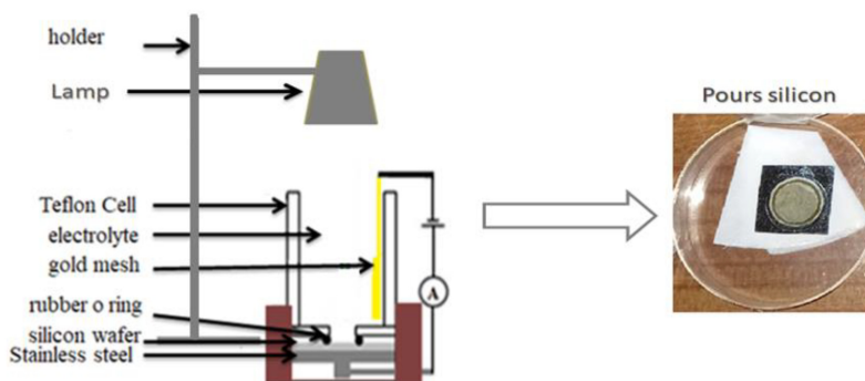
Fig. 1. Setup for the experiment of photo electrochemical etching system.
