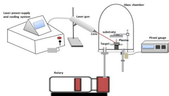
Fig. 2. Setup for the experiment of PLD system.
