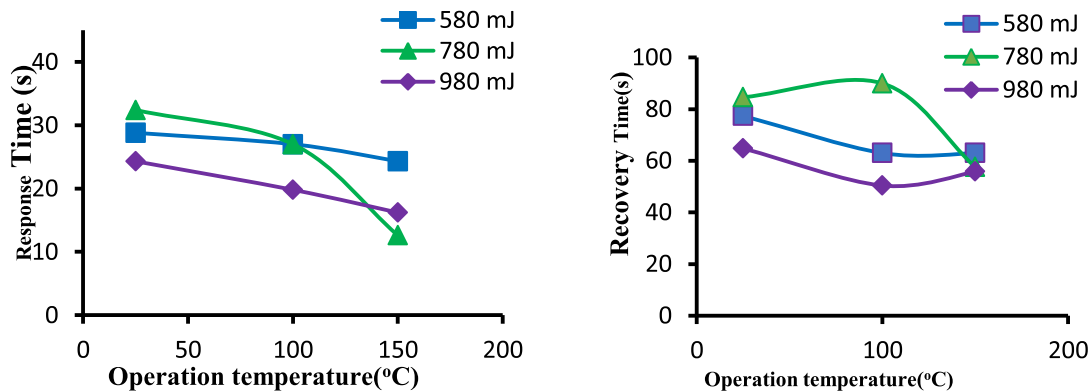
Fig. 9. The fluctuation of response time and recovery time of the NiO NPs at varied operation temperatures and laser pulse energy at 1064 nm.
