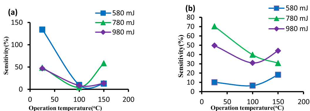
Fig. 8. The fluctuation of sensitivity at varied operation temperatures for NiO NPs/PS samples created at different laser pulse energy for a. 1064 nm and b.355 nm.
