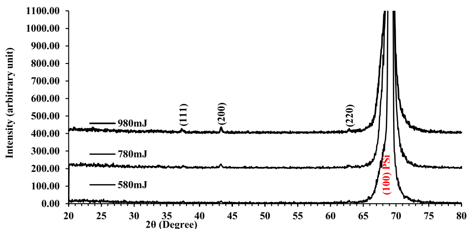
Fig. 4. The X-ray diffraction peaks of NiO grown on Ps substrate with different laser pulse energies and an Nd: YAG laser 355 nm.
