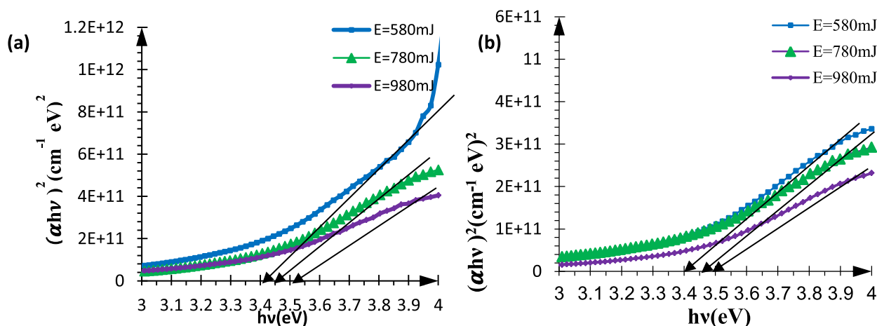
Fig. 7. The relationship between (\alpha h\nu)^2 versus h\nu for NiO thin films prepared by PLD technique for a. 1064 nm and b.355 nm.
