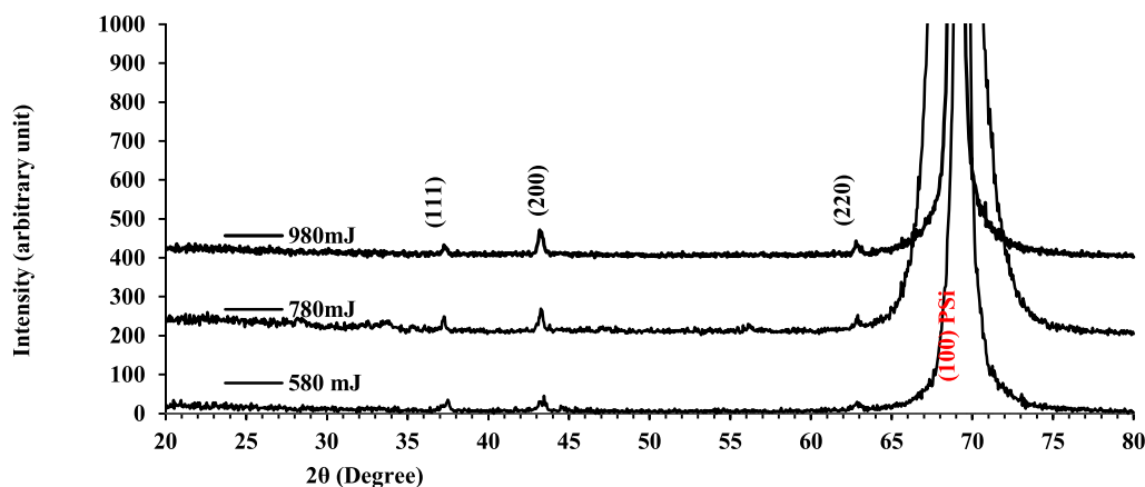
Fig. 3. The X-ray diffraction peaks of NiO grown on Ps substrate with different laser pulse energies and an Nd: YAG laser 1064 nm.
