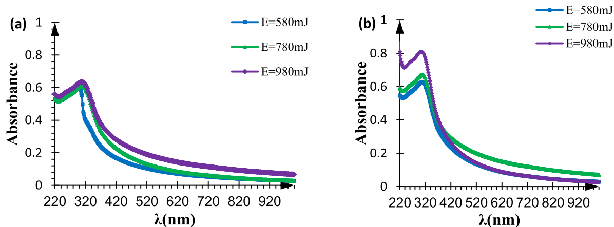
Fig. 5. The relationship between absorption fluctuation and wavelength for NiO grown on glass substrate for Nd: YAG laser a. 1064 nm and b. 355 nm.
