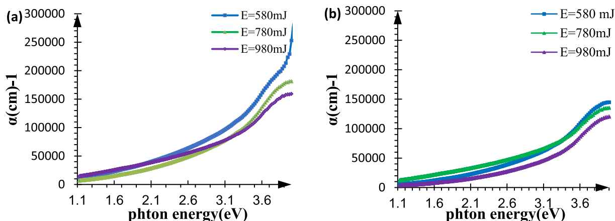
Fig. 6. The relationship between the absorption coefficient fluctuation and photon energy for NiO grown on glass substrate at Nd: YAG laser for a. 1064 nm and b. 355 nm.
