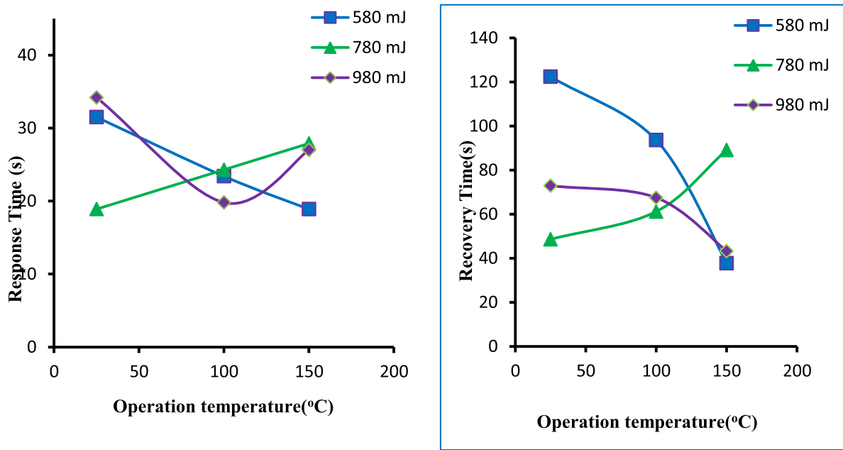
Fig. 10. The fluctuation of response time and recovery time of the NiO NPs at varied operation temperatures and laser pulse energy at 355 nm.
